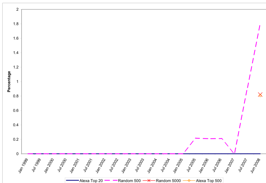
Fig. 6 XHTML 1.1 Strict (Lines represent Archive, circle and cross represent Ground Truth)
