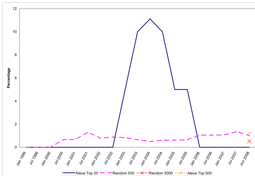
Fig. 9 VBScript (All Versions – Lines represent Archive, circle and cross represent Ground Truth)
