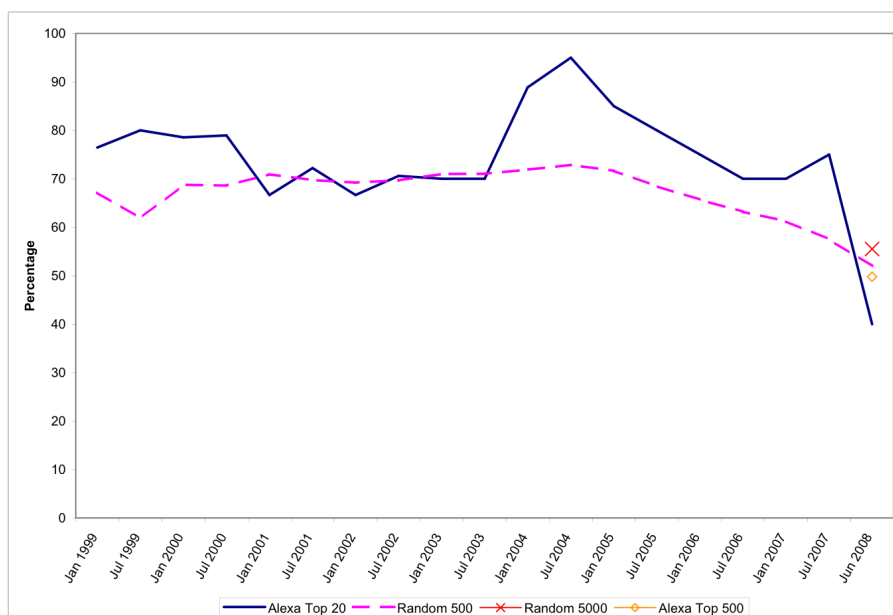
Fig. 4 HTML 4 (versions 4 and 4.01 – Lines represent Archive, circle and cross represent Ground Truth)
