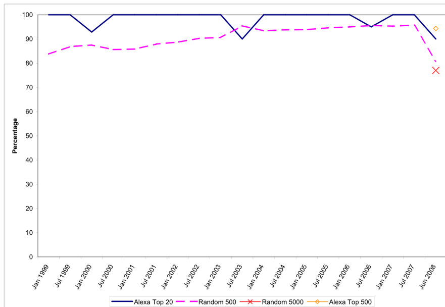
Fig. 8 JavaScript (All Versions – Lines represent Archive, circle and cross represent Ground Truth)
