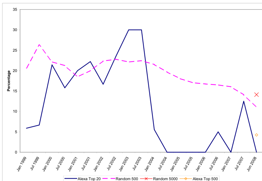
Fig. 2 HTML 2 (Lines represent Archive, circle and cross represent Ground Truth)
