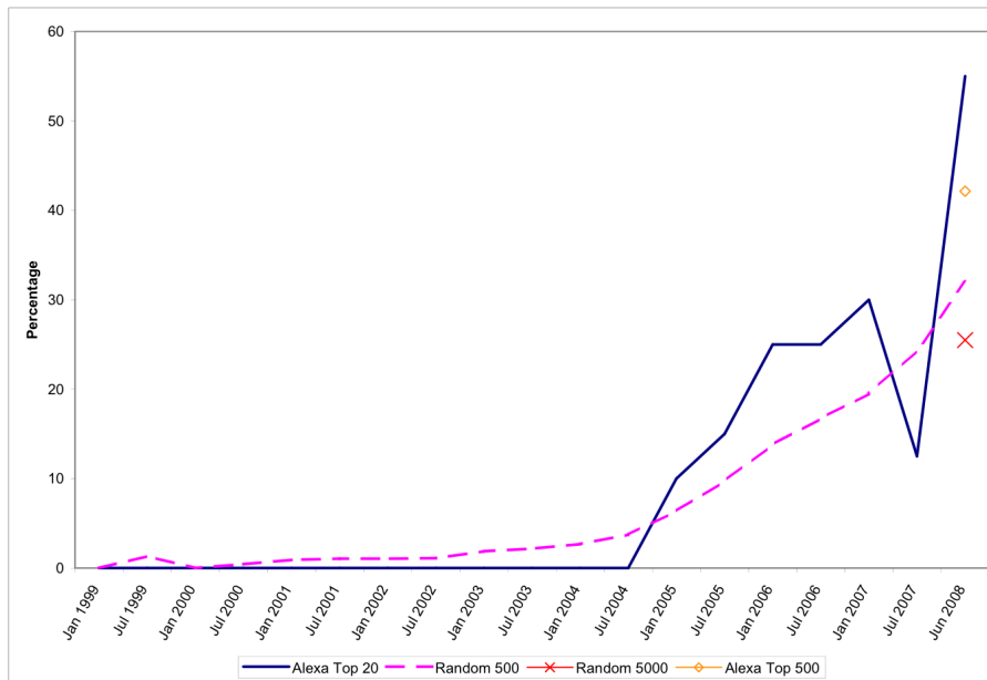
Fig. 5 XHTML 1.0 (Lines represent Archive, circle and cross represent Ground Truth)
