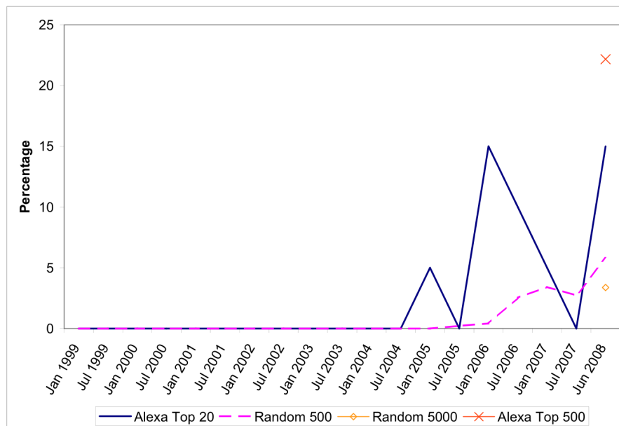
Fig. 11 AJAX / XMLHttpRequest (Lines represent Archive, circle and cross represent Ground Truth)
