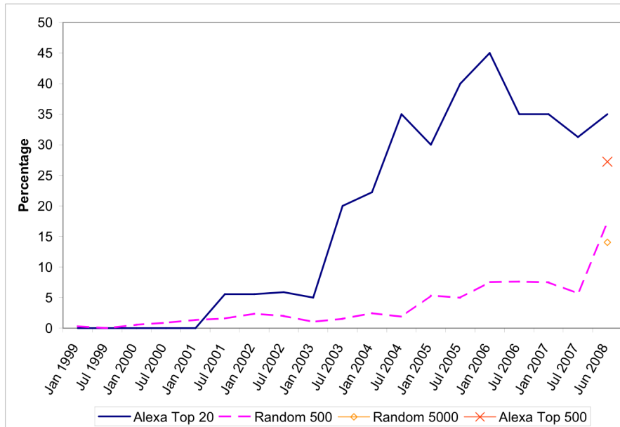
Fig. 10 AJAX / iFrame (Lines represent Archive, circle and cross represent Ground Truth)
